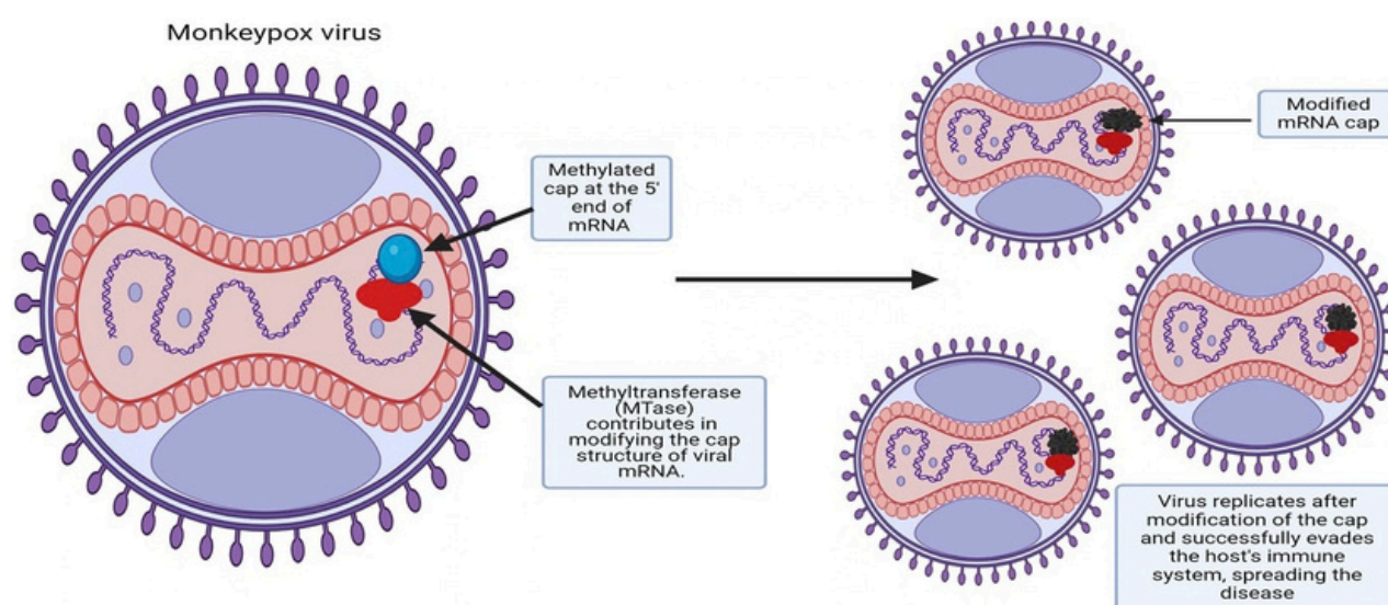
Figure 1. Monkeypox virus structure and the role of mRNA cap methylation. Methyltransferase-mediated modification of the 5' cap of viral mRNA supports transcript stability and cap-dependent translation. This modification allows viral mRNA to evade cytoplasmic innate immune sensing, permitting productive replication. The responsible enzymes are identified in Table 1. Image created with BioRender.com.
