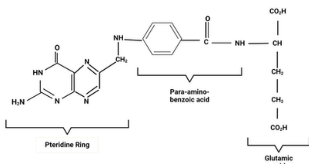
Figure 2. Chemical structure and physiological state of folic acid (N-pteroyl-L-glutamic acid). It comprises a pteridine ring linked to p-aminobenzoic acid, which is bound via an amide bond to L-glutamic acid. At physiological pH, both glutamate carboxyl groups are ionized, resulting in a dianionic molecule with a high topological polar surface area. Image created with BioRender.com.
