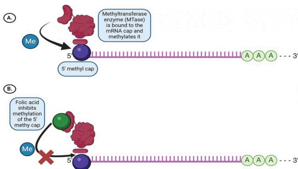
Figure 3. Proposed mechanism of folic acid interference with orthopoxvirus mRNA cap methylation. (A) A SAM-dependent cap methyltransferase methylates the 5' cap of viral mRNA. (B) Hypothesized mechanism in which folic acid occupies the enzyme active site, preventing methyl transfer and leaving viral transcripts susceptible to detection by cytoplasmic innate immune sensors. This figure depicts a hypothesis derived solely from molecular docking (12); it does not represent a demonstrated enzymatic result, and no biochemical assay has yet verified this mechanism. Image created with BioRender.com.
